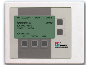
Programmer (external) for automatic control L x W x D (mm): 158 x 125 x 32
